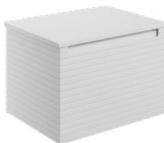
WALL HUNG 600MM 1 DRAWER BASIN UNIT & TOP W600 x H413 x D460mm
