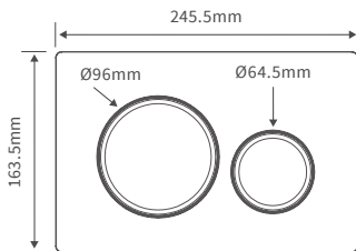
ROUND FLUSHPLATE
