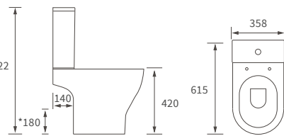
RIMLESS CLOSE COUPLED PAN AND CISTERN OPEN BACK
